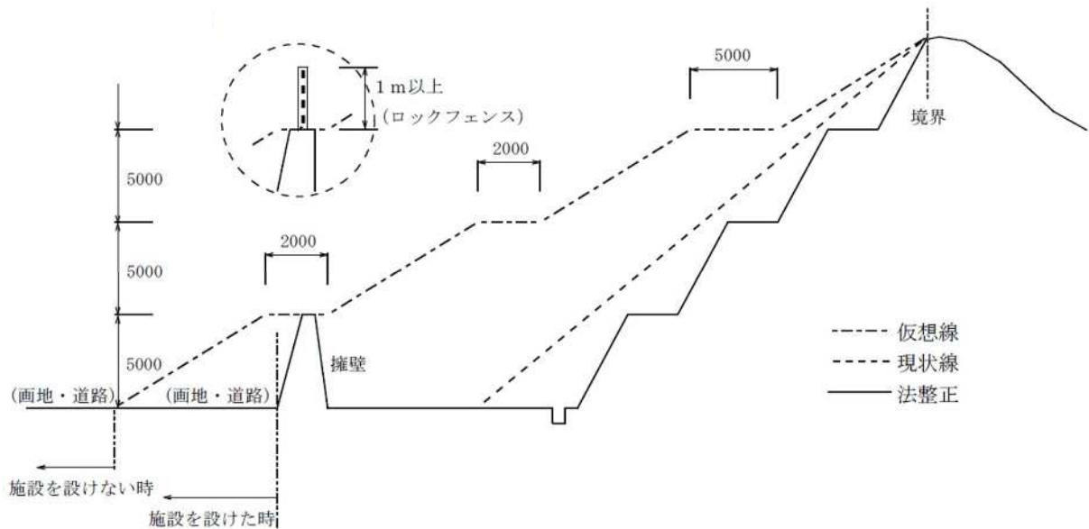
図3-35
